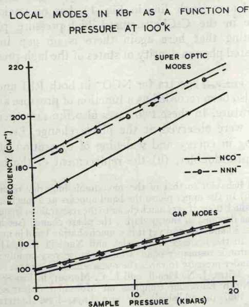
FIG. 15. Comparison of the pressure dependence of the local-mode frequencies of \text{NCO}^- and \text{N}_3^- in the low-pressure phase of KBr at 100°K.
